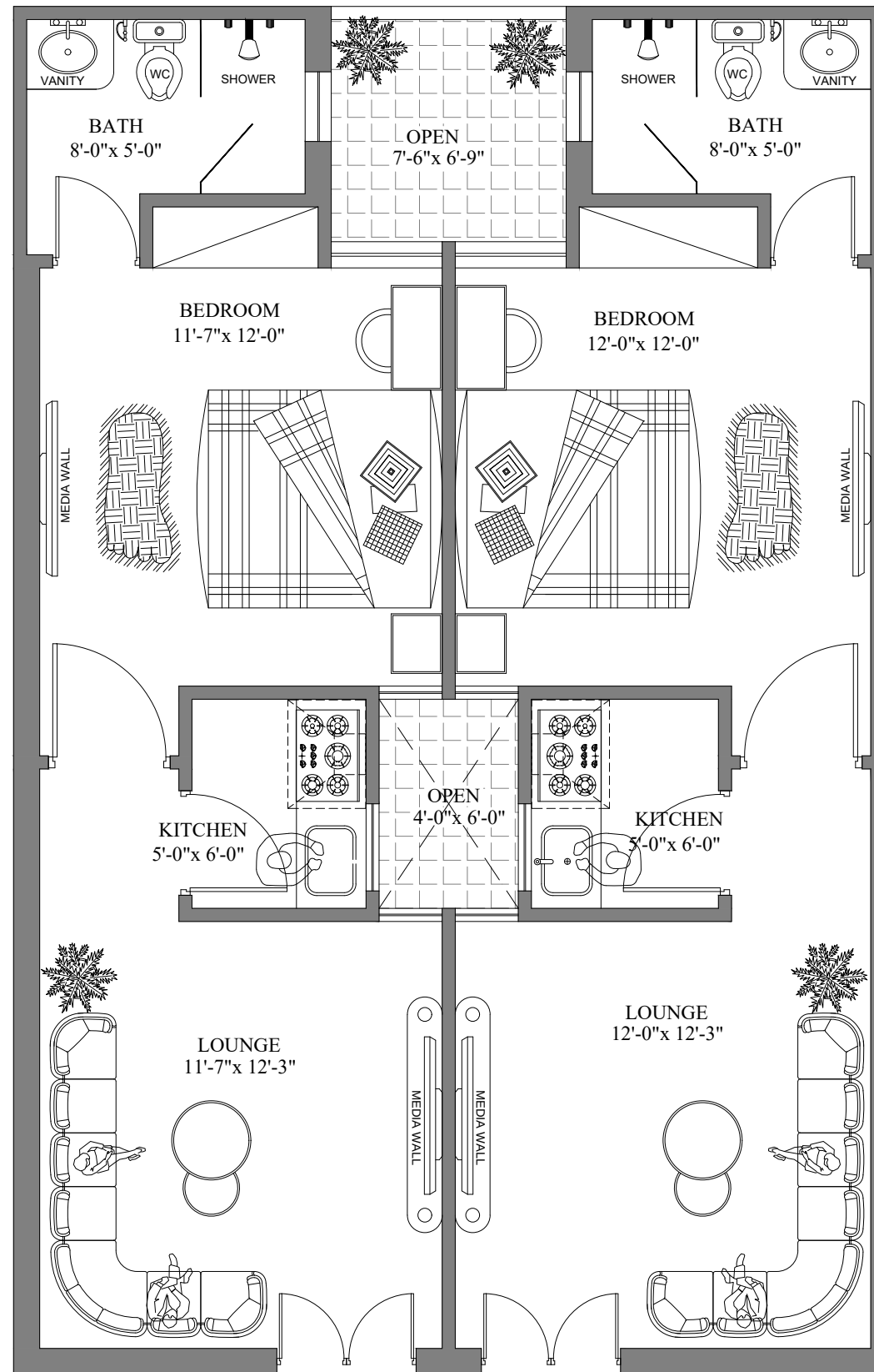
GROUND FLOOR LAYOUT PLAN
